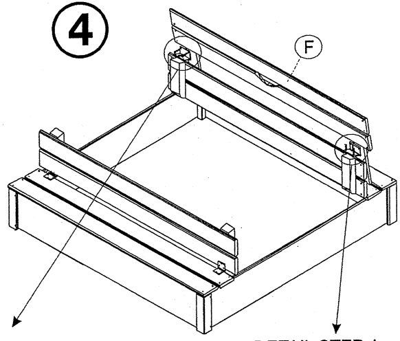
DETAIL STEP 4
