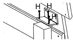
DETAIL STEP 4
